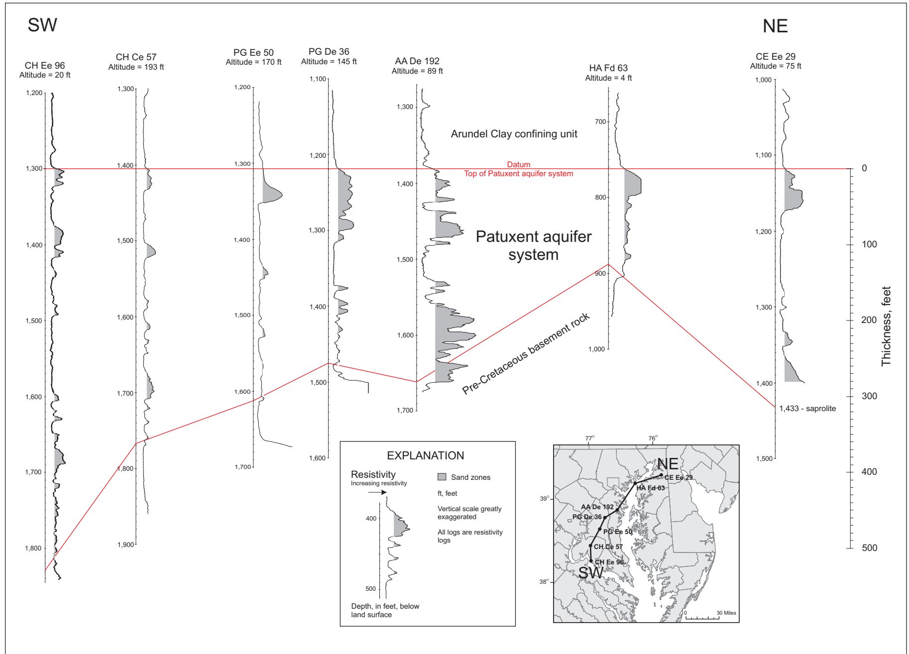
Hydrostratigraphic cross section showing thickness and sand content of the Patuxent aquifer system along strike.
